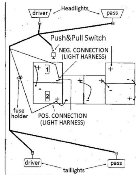
Club Car Basic 36-volt Wiring Diagram
