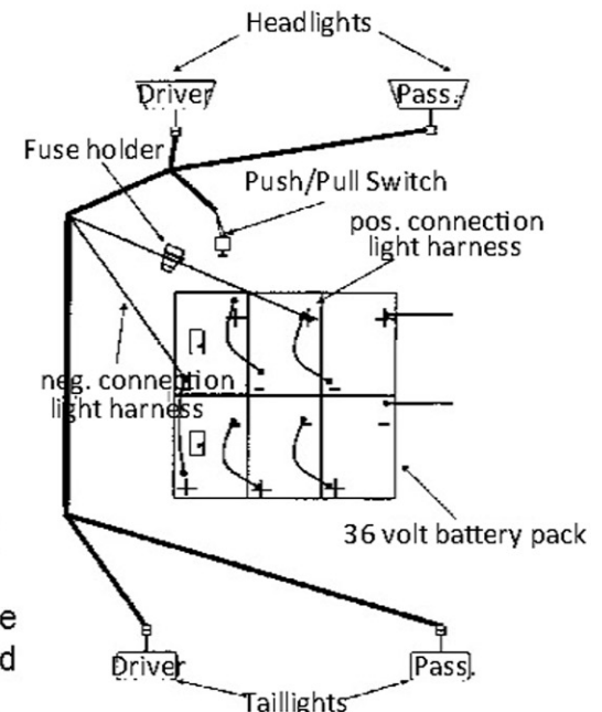
EZGO Basic 36-volt wiring Diagram
